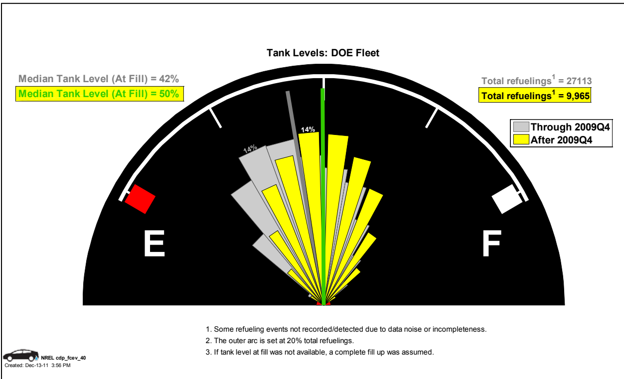
Figure 117: Hydrogen tank level at fueling (CDP40)
