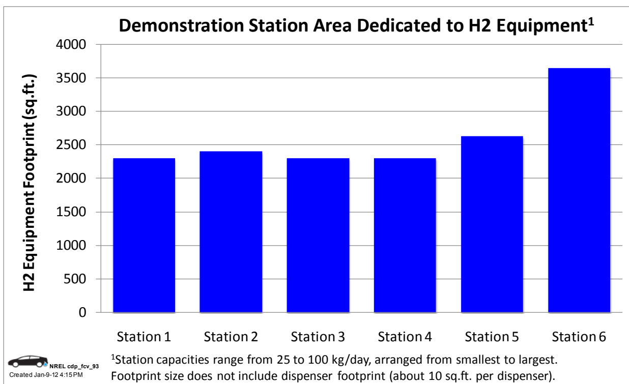
Figure 125: Demonstration hydrogen station equipment footprint (CDP93)
