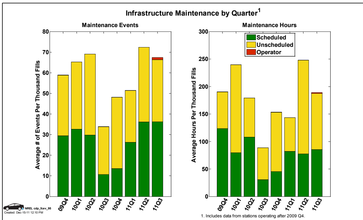
Figure 104: Infrastructure maintenance by quarter after 2009Q4 (CDP95)
