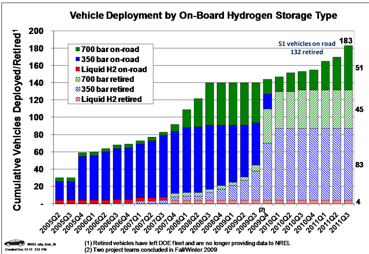
Figure 6: Cumulative number of vehicles deployed, by hydrogen storage type and status (CDP25)
